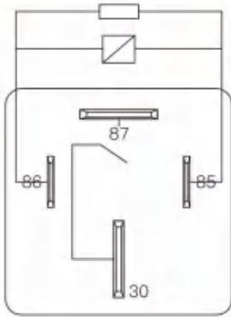
常开A型/Normally open A type
