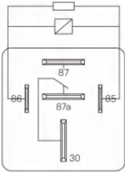
转换C型/Conversion C type
