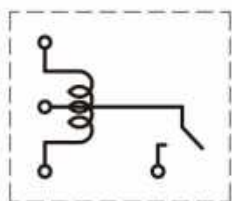
常开A型/Normally open A type
