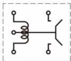
常开U型/Normally open U type
