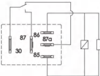
转换C型/Conversion C type
