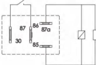
常开A型/Normally open A type
