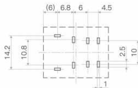
安装孔图(底视图) Installation hole drawing(Bottom view)
