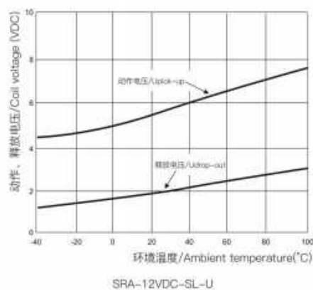
动作、释放电压温度特性 Pick-up & drop-out voltage-ambient temperature characteristic
