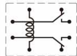
2转换2C型/Conversion 2C type
