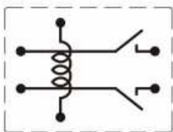
2常开2A型/Normally open 2A type
